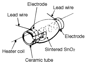
Fig. 1 - Sensor structure
