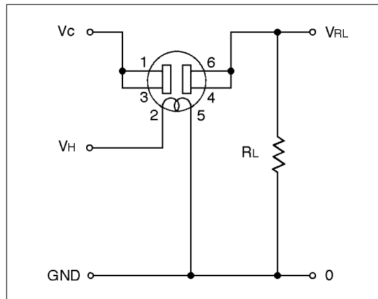
Fig. 2 - Basic measuring circuit
