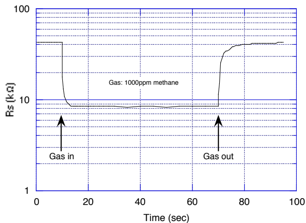
Fig. 9 - Response speed
