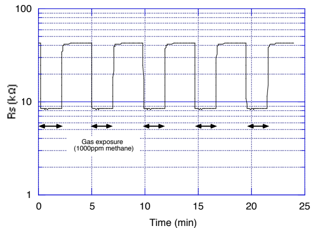
Fig. 10 - Repeatability
