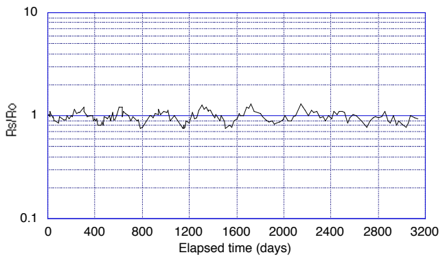
Fig. 12 - Long term stability ( R_0 = R_s on day 1)
