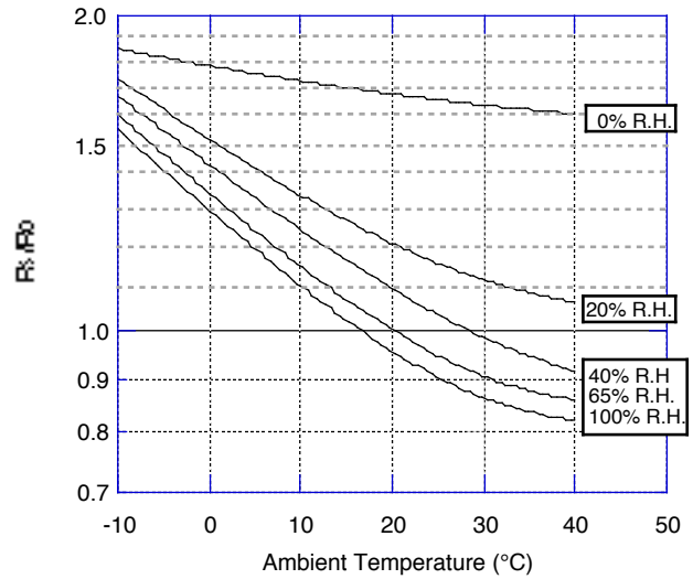
Fig. 6 - Temperature and humidity dependency ( R_s/R_o )
