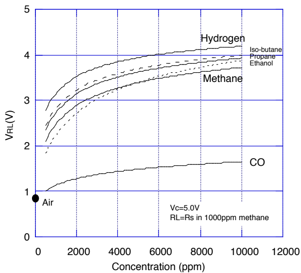
Fig. 5 - Sensitivity to various gases ( V_{RL} )
