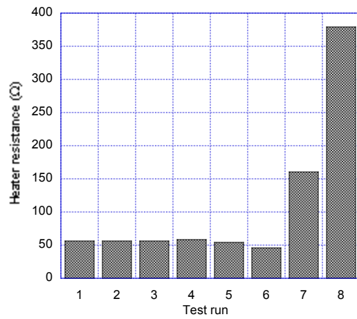
Fig. 18 - Short-term effect of V_H on R_H
