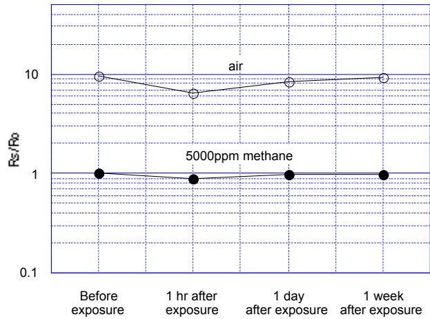
Fig. 19a - Durability to HMDS exposure for TGS2611-C ( R_0 = R_s in 5000ppm methane before exposure)
