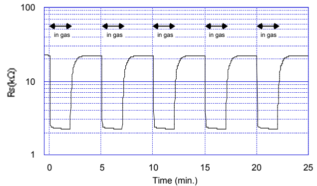
Fig. 11 - Repeatability
