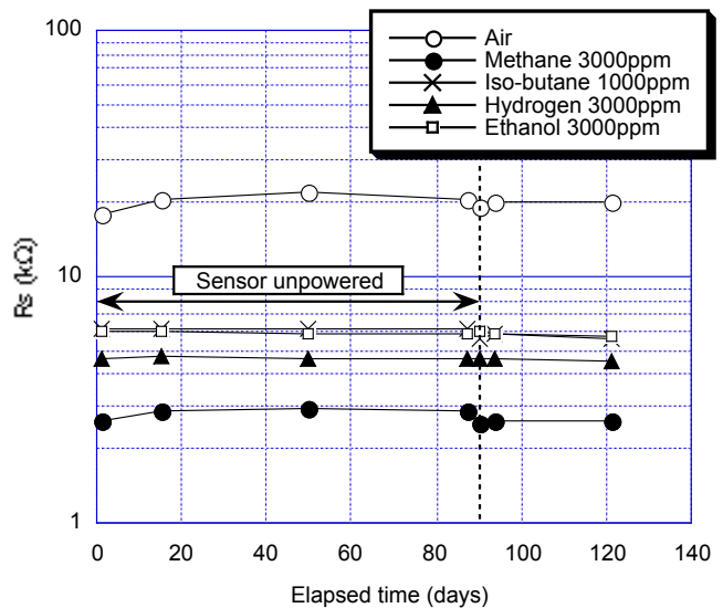
Fig. 14 - Influence of unenergizing on TGS2611-C
