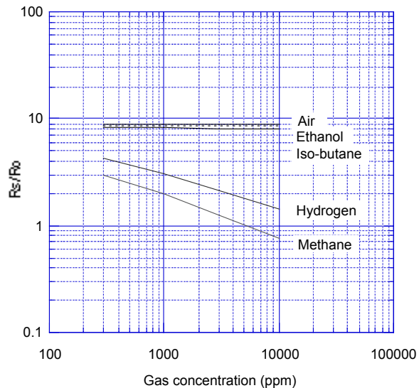
Fig. 4b - Sensitivity to various gases ( R_s/R_o ) of TGS2611-E
