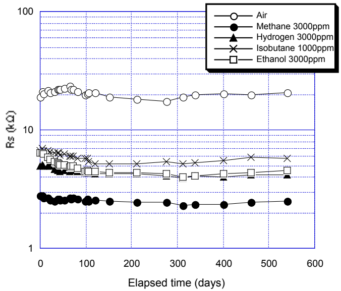
Fig. 13 - Long-term stability (continuous energizing) of TGS2611-C
