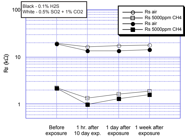
Fig. 15 - Corrosion test of TGS2611-C
