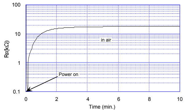
Fig. 12 - Initial action
