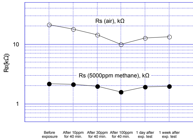
Fig. 19b - Durability to HMDS exposure for TGS2611-C
