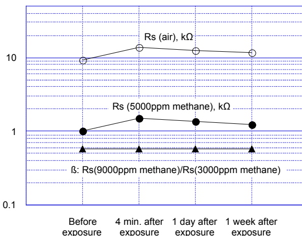
Fig. 20 - Lighter gas exposure test of TGS2611-C
