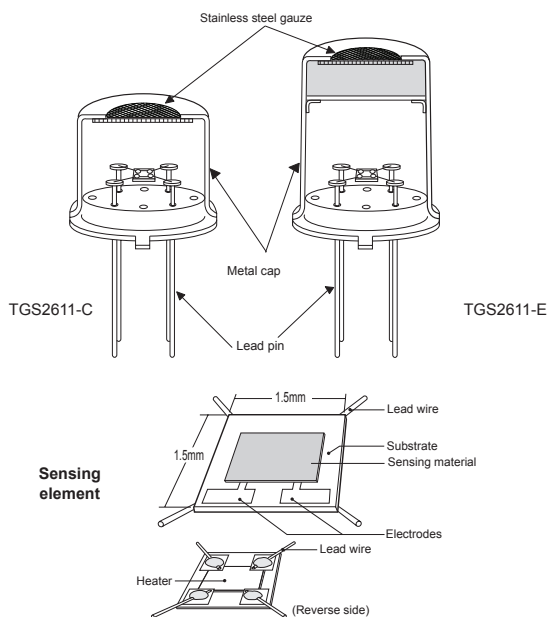
Fig. 1 - Sensor structure
