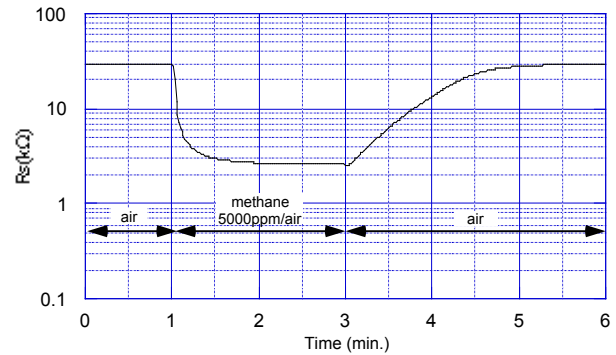
Fig. 10b - Gas response to methane of TGS2611-E
