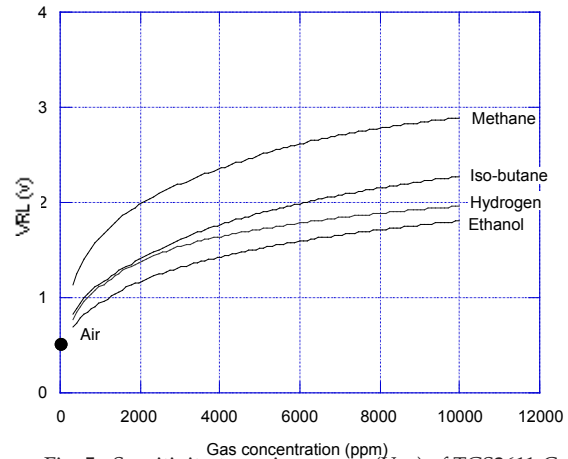
Fig. 5 - Sensitivity to various gases ( V_{RL} ) of TGS2611-C
