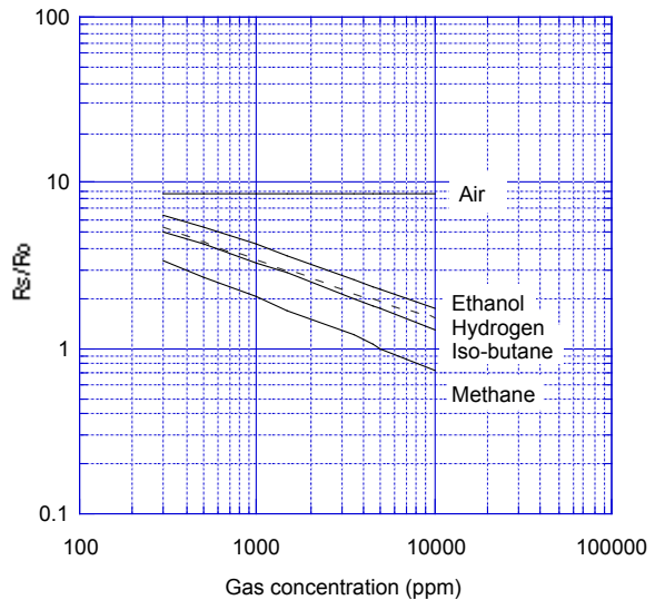
Fig. 4a - Sensitivity to various gases ( R_s/R_o ) of TGS2611-C
