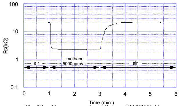
Fig. 10a - Gas response to methane of TGS2611-C
