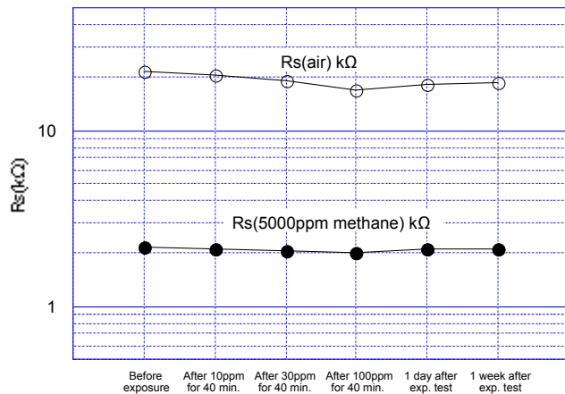
Fig. 19c - Durability to HMDS exposure for TGS2611-E
