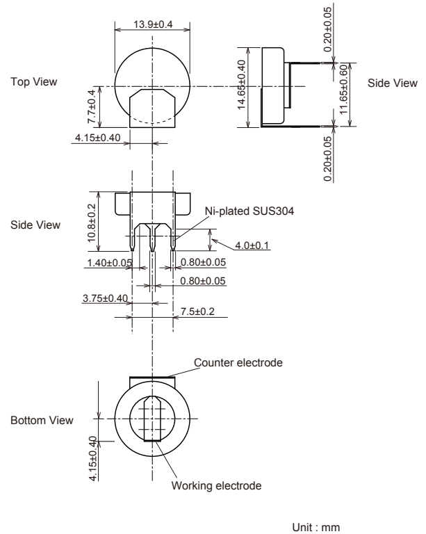
Figure 22 - Dimensions (w/lead pins)
