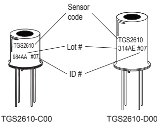
Fig. 1 - Sensor markings
